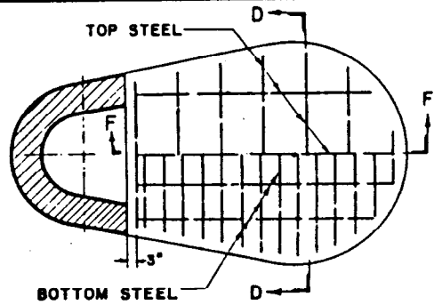
SECTION E-E
