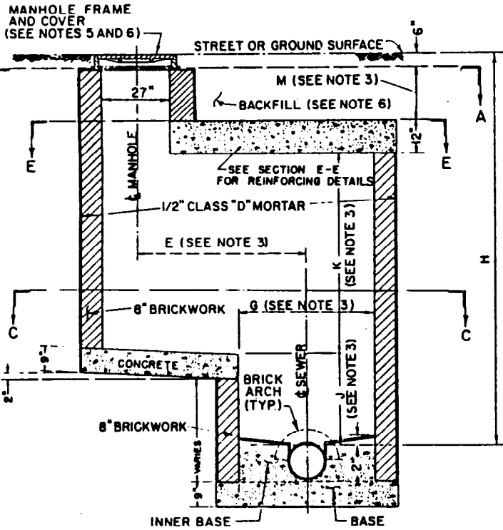
SECTION B-B
