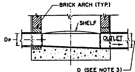
SECTION G-G
