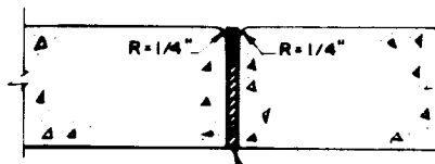
PREMOLDED EXPANSION JOINT FILLER PER SUBSECTION 20I-3.2
