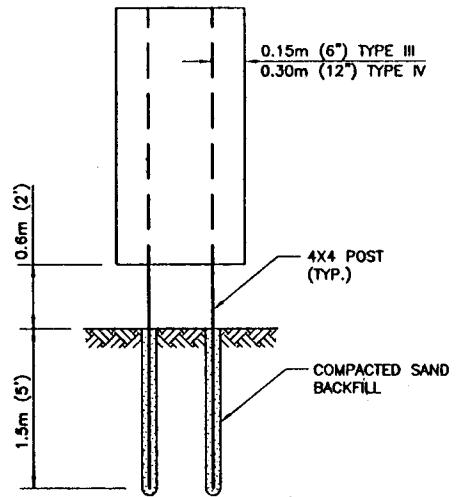
TYPICAL MOUNTING DETAILS
